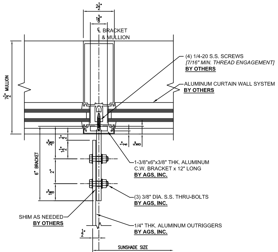
01 END CONNECTION DETAIL AT CURTAIN WALL
