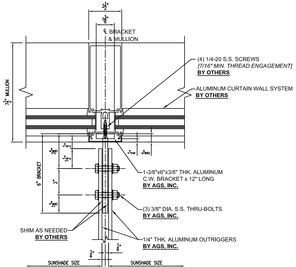
02 INTERMEDIATE CONNECTION DETAIL AT CURTAIN WALL
