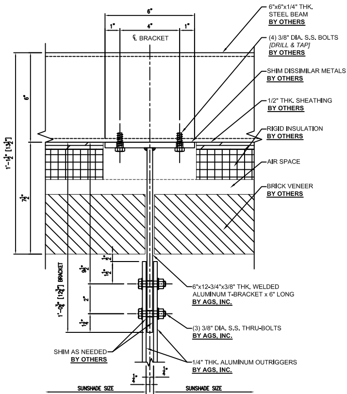
02 INTERMEDIATE CONNECTION DETAIL AT STEEL BEAM
