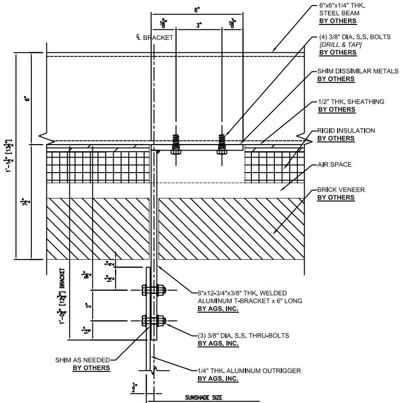
01 END CONNECTION DETAIL AT STEEL BEAM
